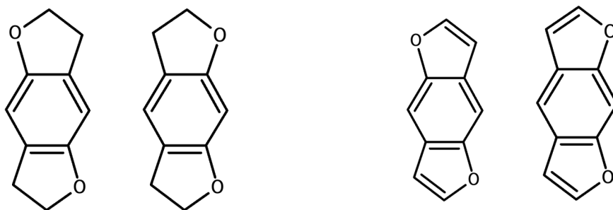
Tetrahydrobenzodifuranil- Benzodifuranil—
