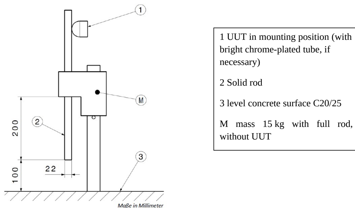
Figure 5: Test fixture (only symbolic)
