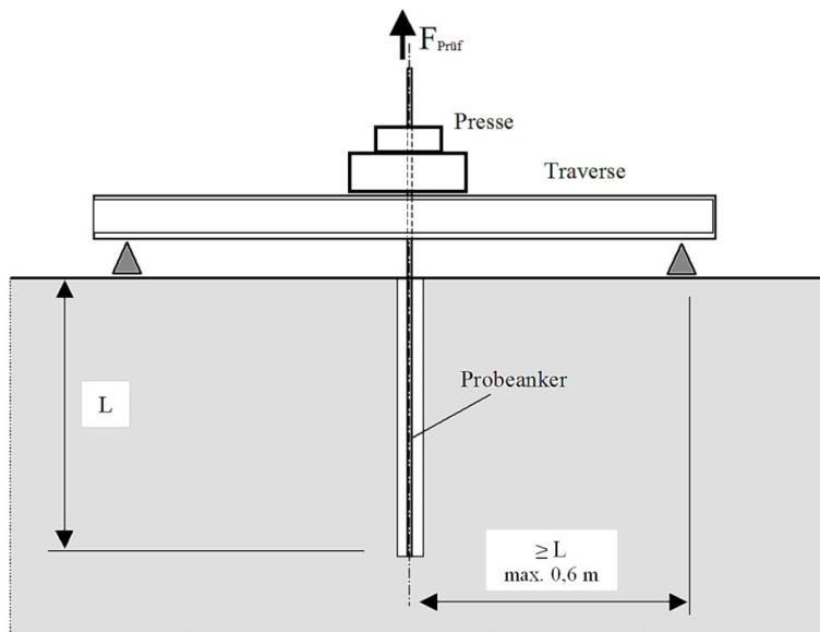
Figure 1: Test arrangement anchor tensile test
