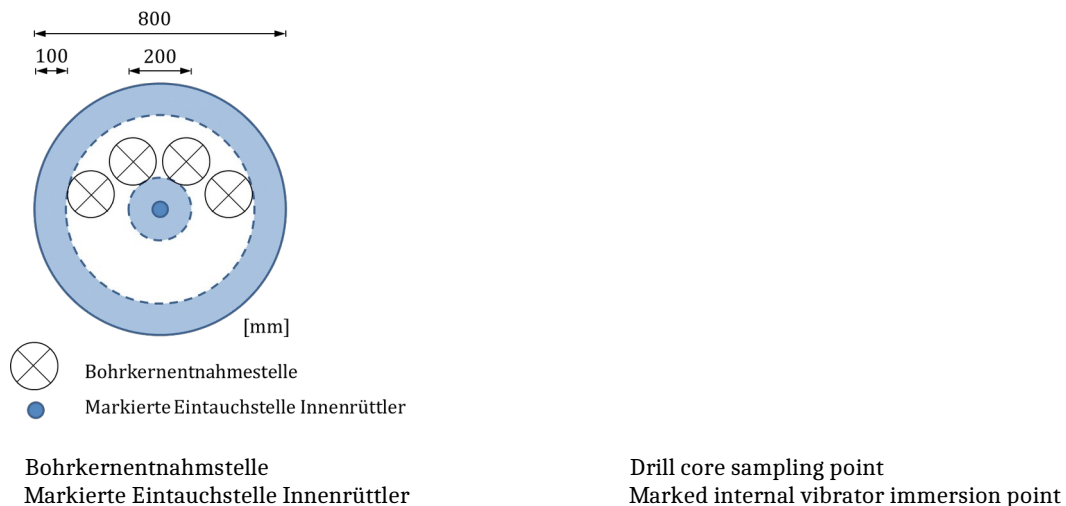
Figure 7: Recommendation for drill core sampling points on the small component (top view)
